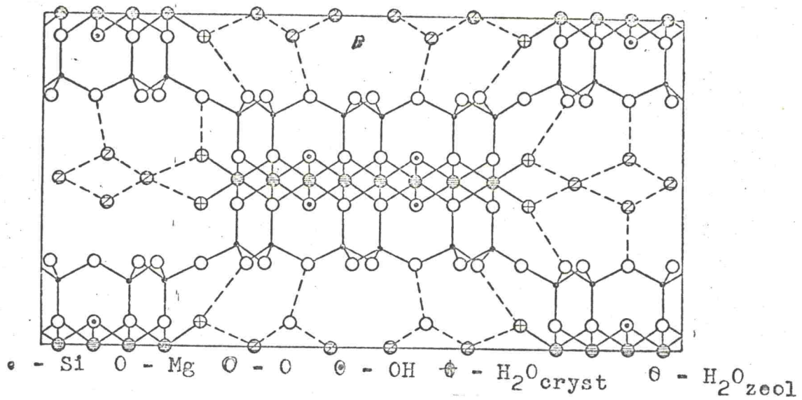
Fig.1. A-unit cell of palygorskite projected on (001)- A
